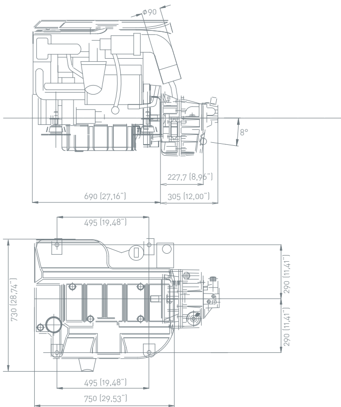
FNM HPE 190 with ZF 45 A gearbox
